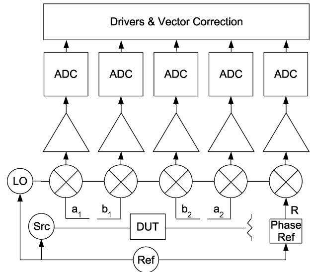
Fig. 1. Block diagram of the measurement system. The hardware consists of five receivers and four directional networks. The receivers measure the incident and reflected waves via the directional networks connected to each port. The fifth receiver measures a phase reference (Phase Ref). The measurement system, source (Src), and phase reference are phase locked to a common reference (Ref).
