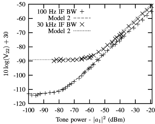
Fig. 10. Comparison of the sample variance V_{22} and the variance predicted by Covariance Model 2. The instrument IF bandwidth was set to 100 Hz and 30 kHz. A low phase-noise signal generator (Agilent E4437) was used to drive the phase reference. For these measurements, the model is able to predict the variance for both wide (30 kHz) and narrow (100 Hz) IF bandwidths.
